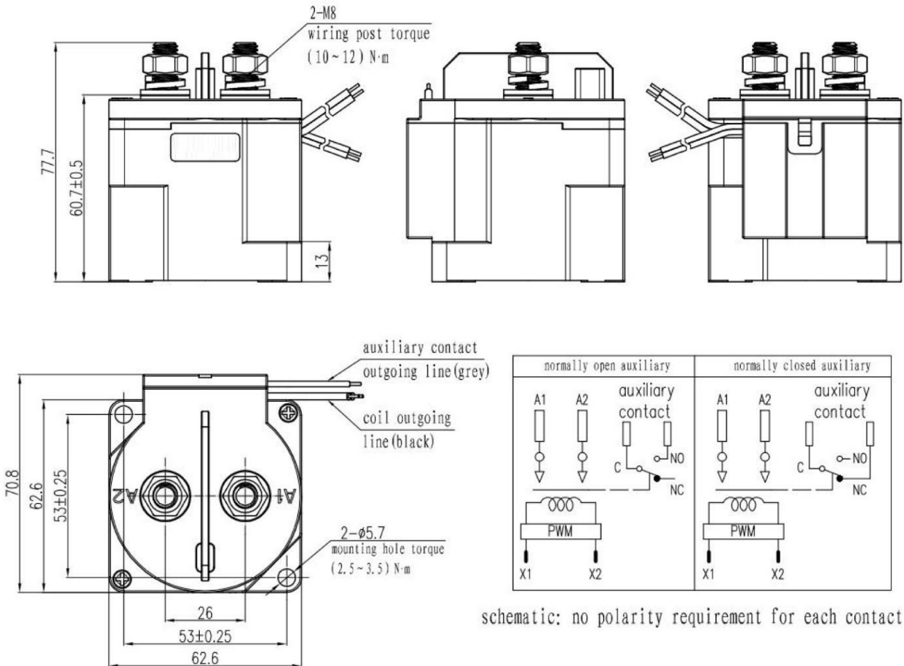
Outline and wiring schematic diagram
